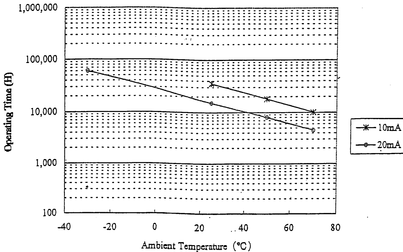
NSPW series White LED (High Power type)
